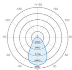
70° Reflector
